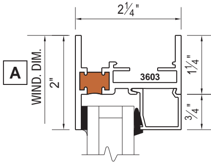
EQUAL LEG (standard)
