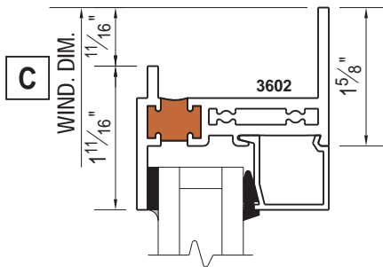
UNEQUAL LEG "Z" (long leg inside)
