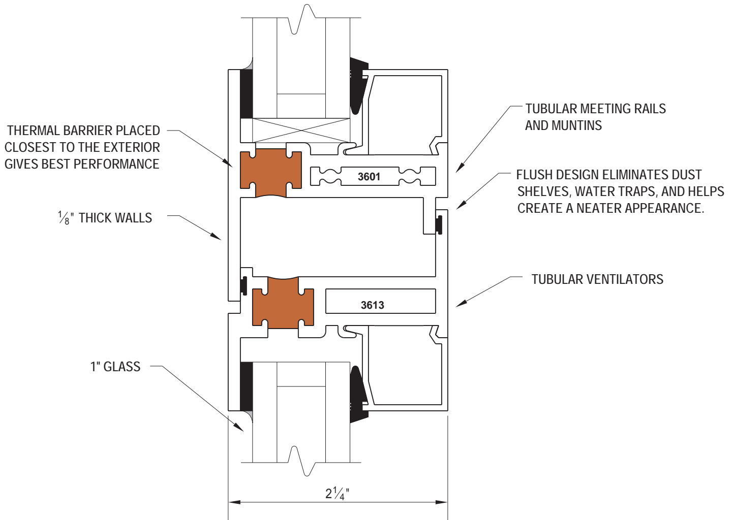
SCALE = FULL SIZE
