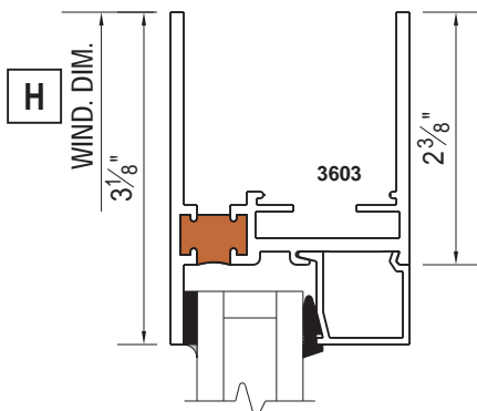
LONG EQUAL LEG (to line up with ventilator)
